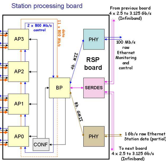
Fig. 4: EMBRACE station processing board
