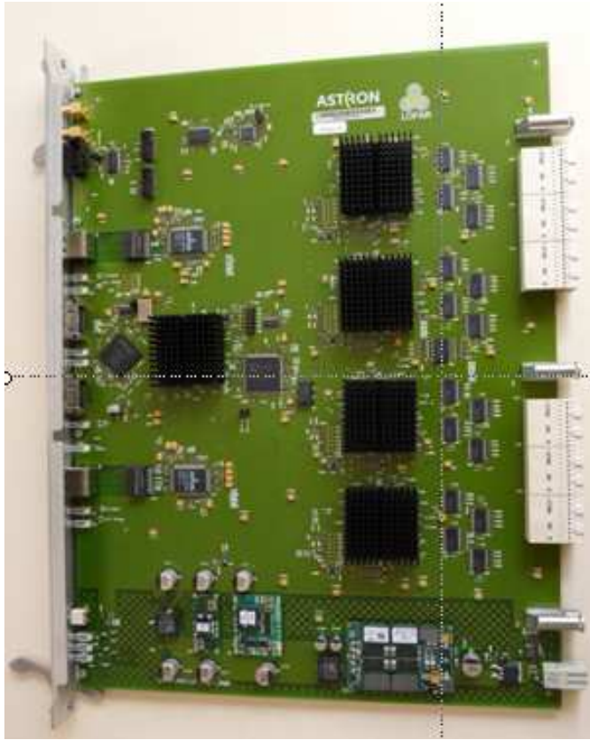
Fig. 2: Board picture
