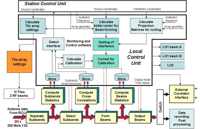
Fig. 5: EMBRACE station processing architecture
