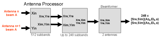
Fig. 3: Antenna processor
